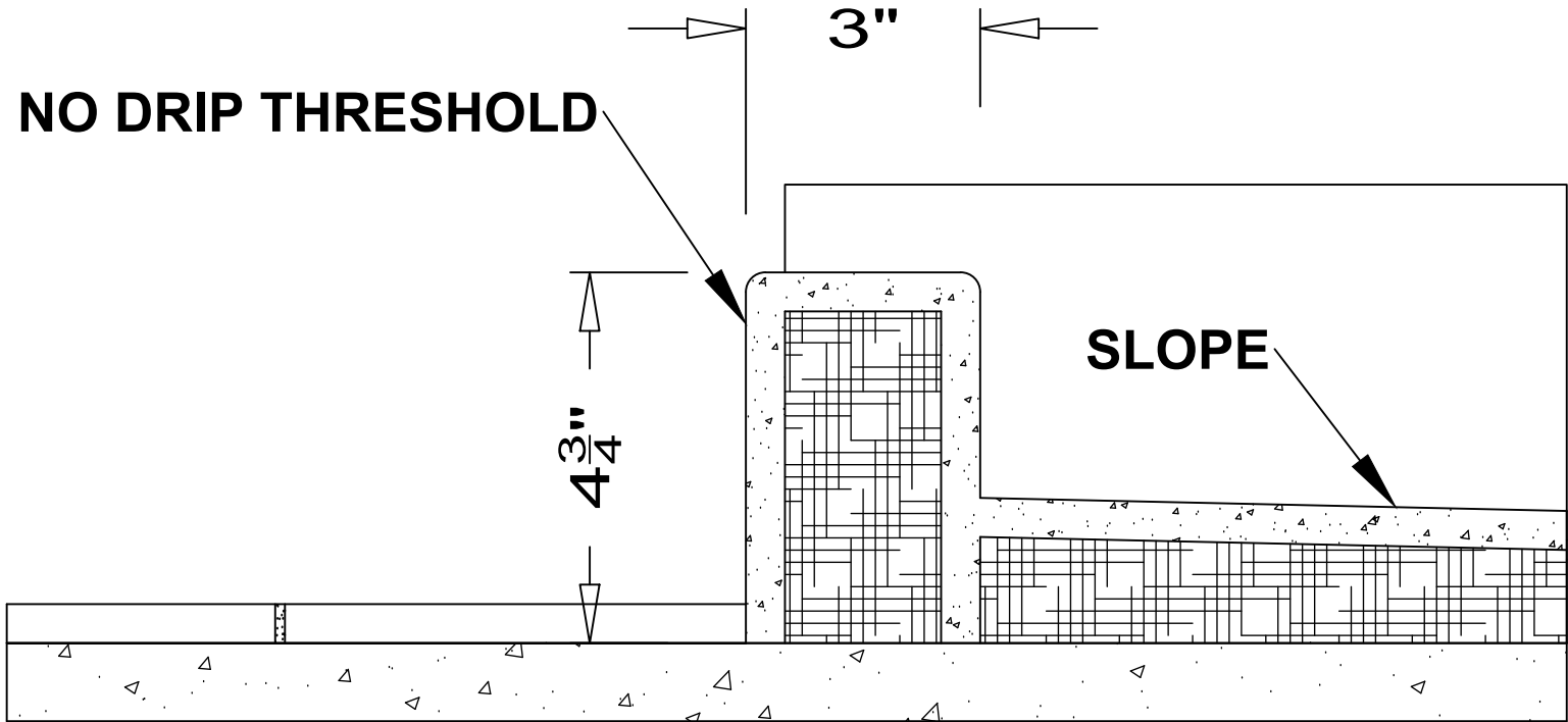
NO DRIP THRESHOLD ENTRY
