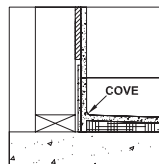
COVED DETAIL COVE OPTION # 3 1/2" WALLS
