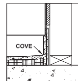
COVED DETAIL COVE OPTION # 2 1/4" WALLS
