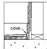
COVED DETAIL COVE OPTION # 4 1/2" WALLS
