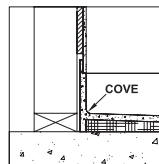
COVED DETAIL COVE OPTION # 1 1/4" WALLS
